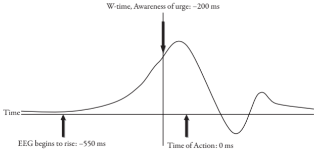
Figure 2.1 Libet's findings.
